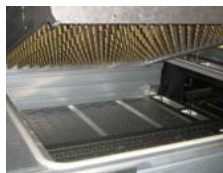
Flexible preheating concept: convection heaters
