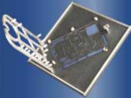
Selective Solder Pallet with hold down canopy
